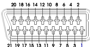
Figure 43.- Scart socket (external view).
